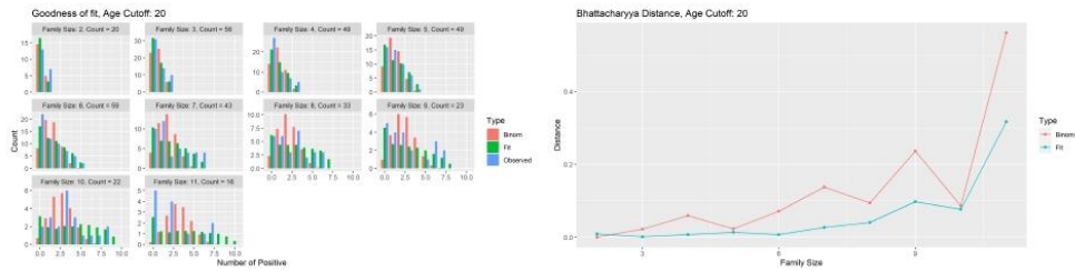
Figure 3: Comparison of distribution of the number of infected cases in households of different sizes in the data to that obtained from the two fitted models, for cutoff age 20 between children and adults.
